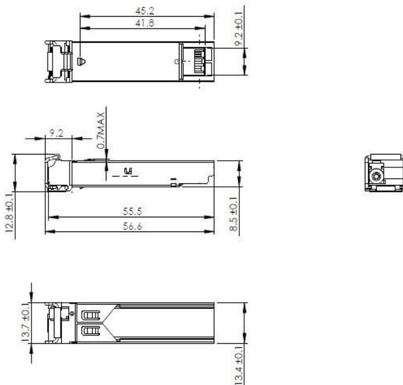
Mechanical Drawing
